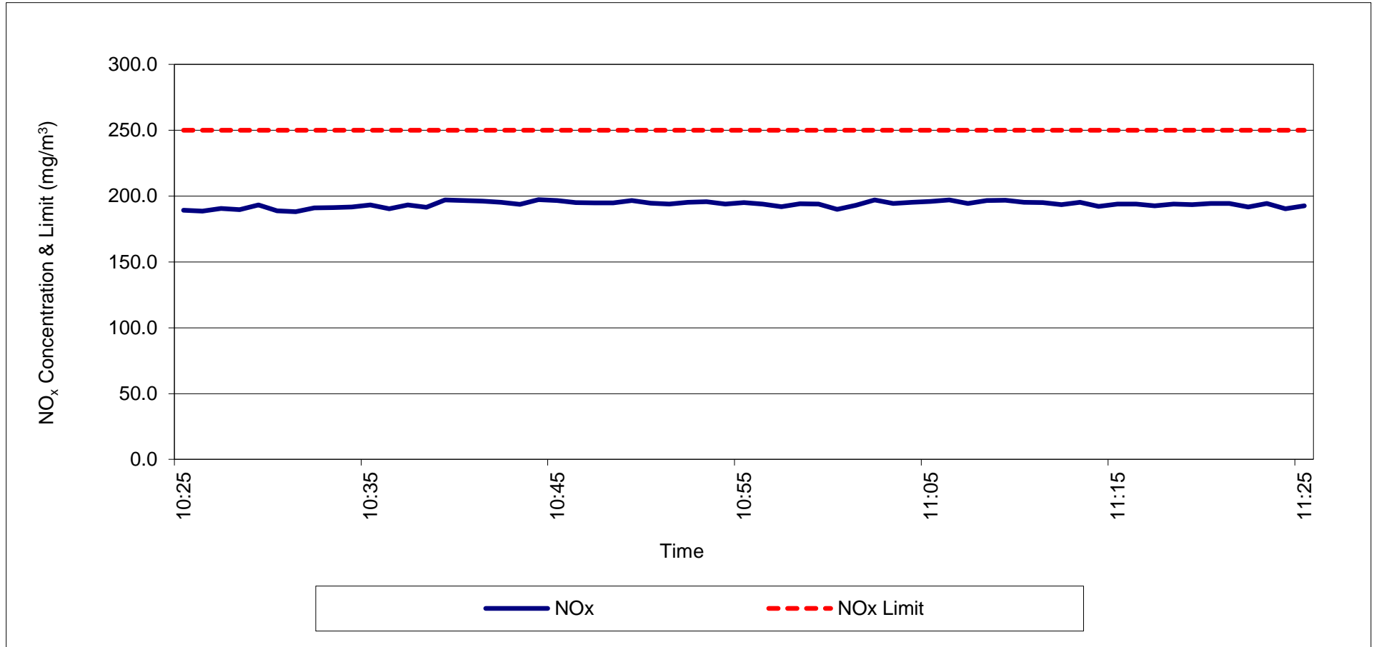
FIGURE B-1 CONTINUOUS LOG OF NITROGEN OXIDES EMISSIONS @ 5% O 2 24 MARCH 2016
